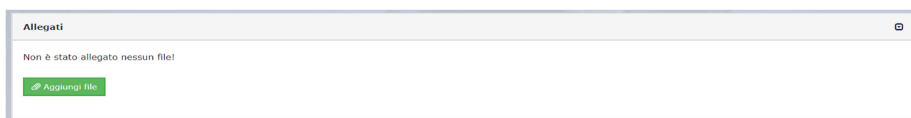
Figura 12 - Allegati (Whistleblower)
